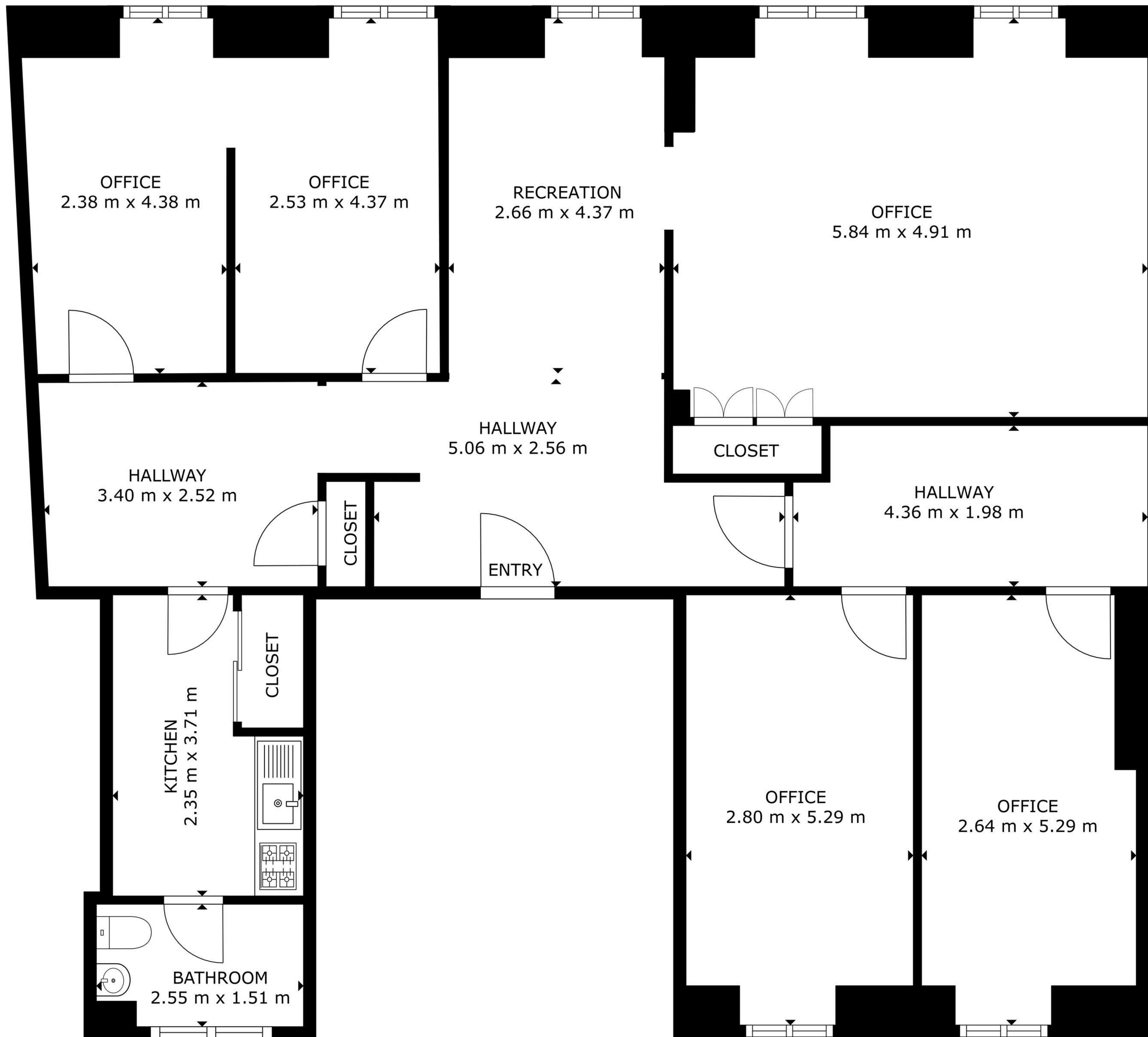
FLOOR PLAN
