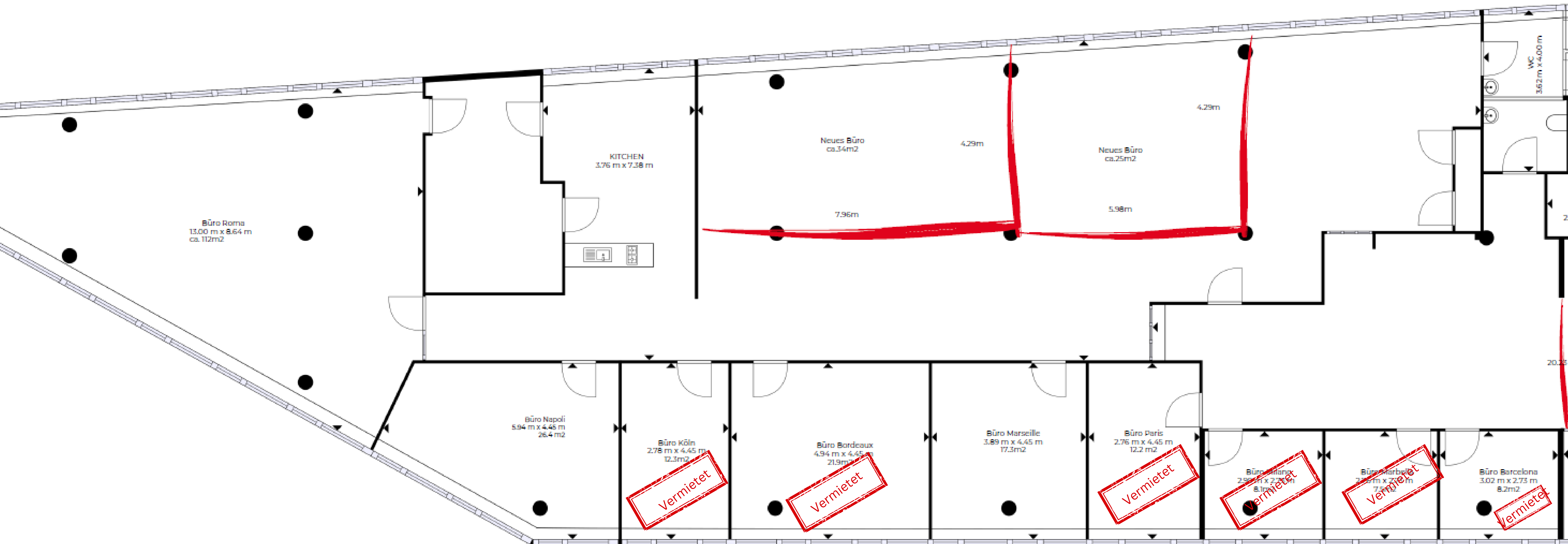
FLOOR PLAN
